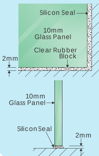
GLASS-TO-FLOOR SEAL
