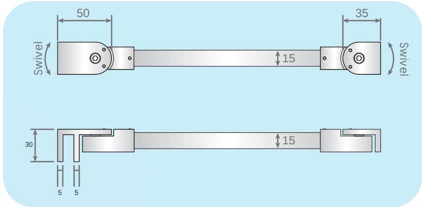
Square Brace Arm 300mm
