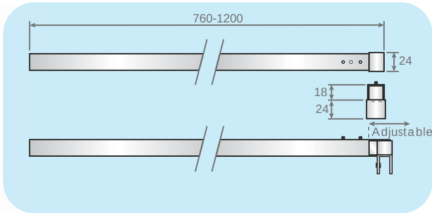
Round Brace Arm Adjustable 760-1200mm
