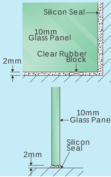
GLASS-TO-FLOOR SEAL
