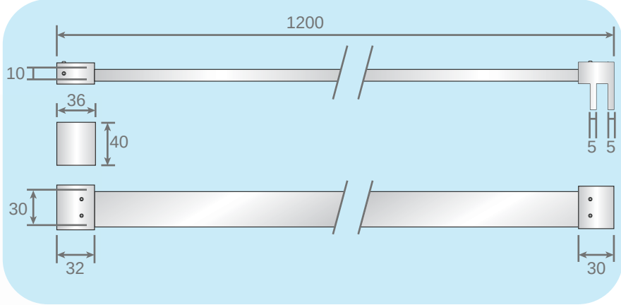
Square Brace Arm 1200mm
