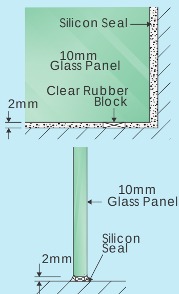
GLASS-TO-FLOOR SEAL
