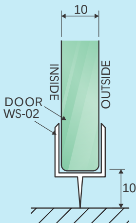
SWING DOOR WATER SEAL
