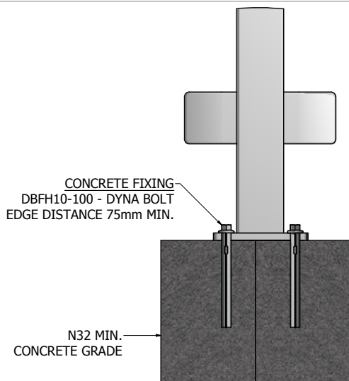
FLANGED POST DETAIL
