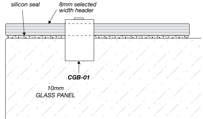
FITTING B
