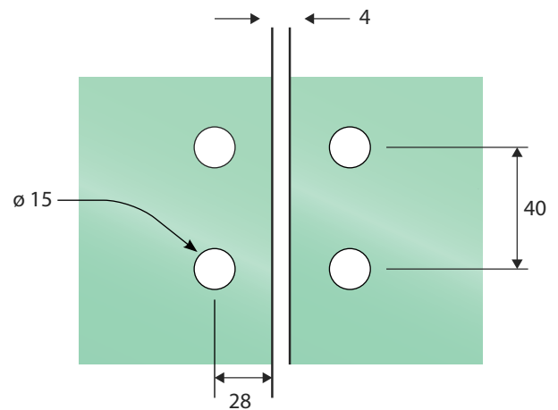
GLASS HOLE DETAIL
