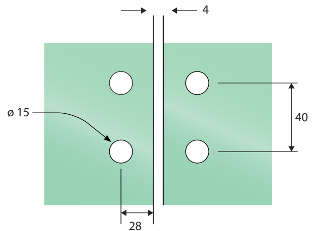
GLASS HOLE DETAIL
