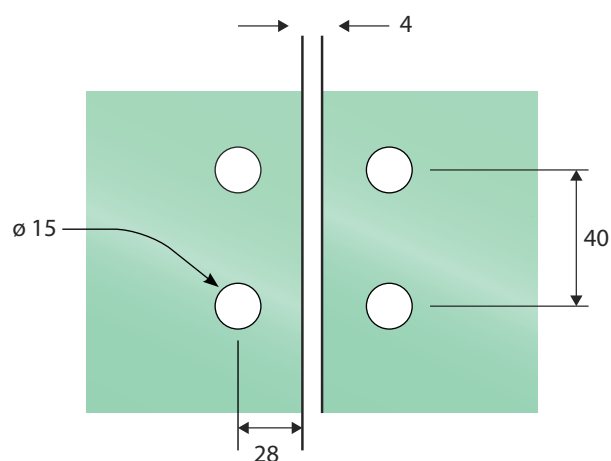
GLASS HOLE DETAIL
