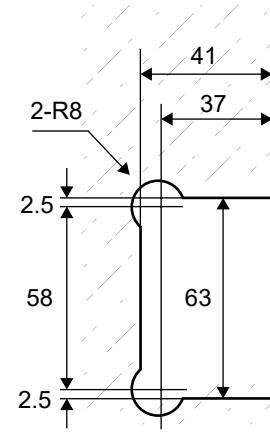
CUT OUT BB
