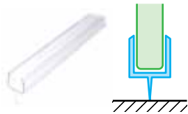
WS-02 Translucent Weather Strip WS-02
