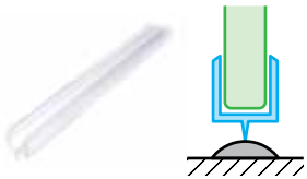
WS-01 Translucent Weather Strip WS-01
